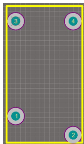
Figure 3 Optocoupler package style
